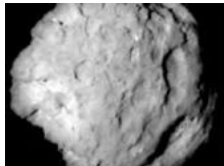
Comet Wild 2
