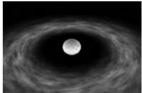
4. Primordial disc spreads around the star resulting in planet formation
