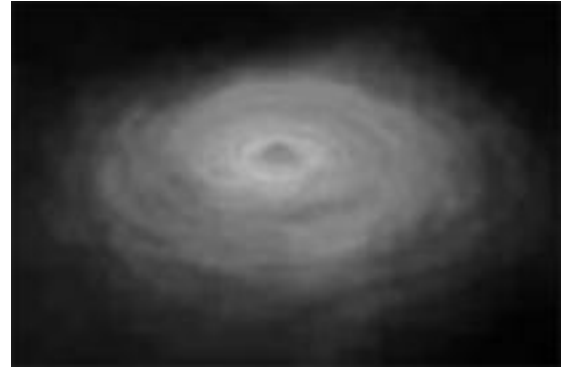
2. Primordial disc of stardust
