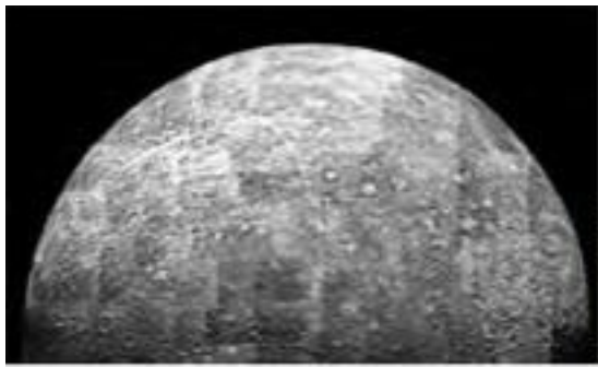
Planet Mercury
