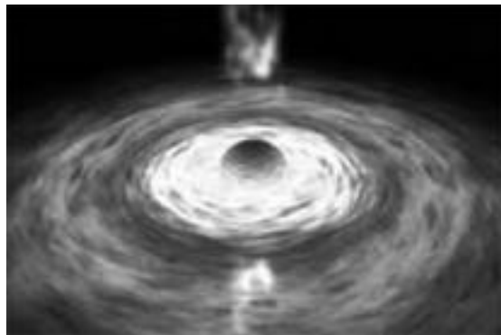
3. Nuclear fusion blows away the lightest materials creating space for planets to develop.
